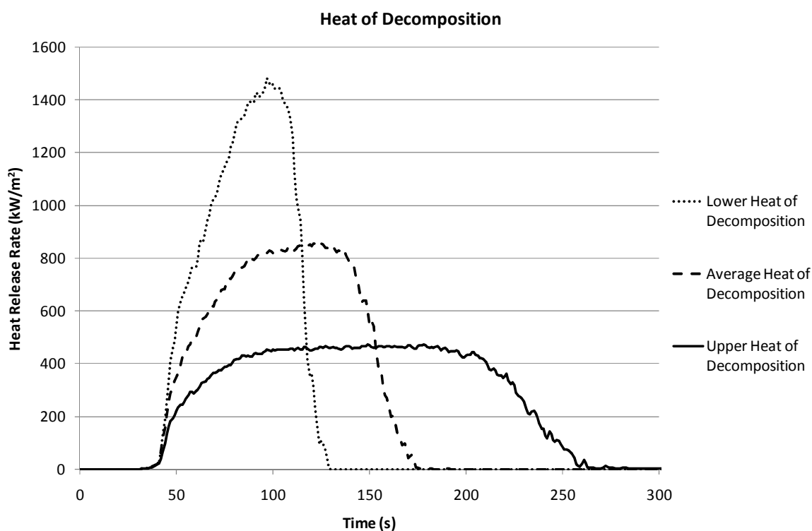
Figure 8. Effect of Heat of Decomposition on Cone Calorimeter HRR Histories
