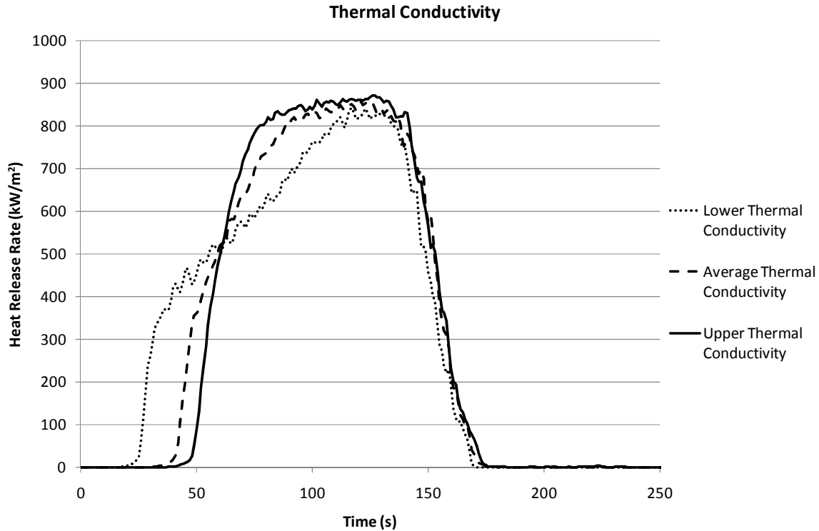
29 30 31 32 Figure 3. Effect of Thermal Conductivity on Cone Calorimeter HRR Histories
